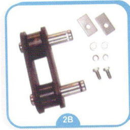
Type ENA-190-5 mercerizing clip and chain. Suitable for the following main equipment: Japan Wakayama Mercerizing Machine
