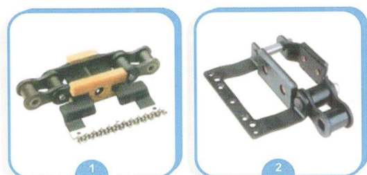
Type ENA-530 vertical chain and pin holder. Suitable for MONFORTS Knitting Stenter
