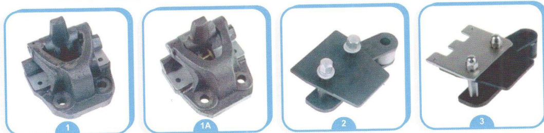
Type ENA-190-3 mercerizing clip and chain. Suitable for the following main equipment: Japan Wakayama Mercerizing Machine
