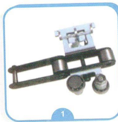
Type ENA-240 chain and pin holder. Suitable for 452 Heat Stenter
