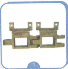
Type ENA-750 vertical chain and pin holder. Suitable for Benniger Mercerzing Stentering Range
