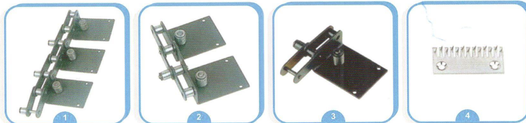
Type ENA-520 chain and pin holder. Suitable for Compact BRUCKNER Vertical Stenter
